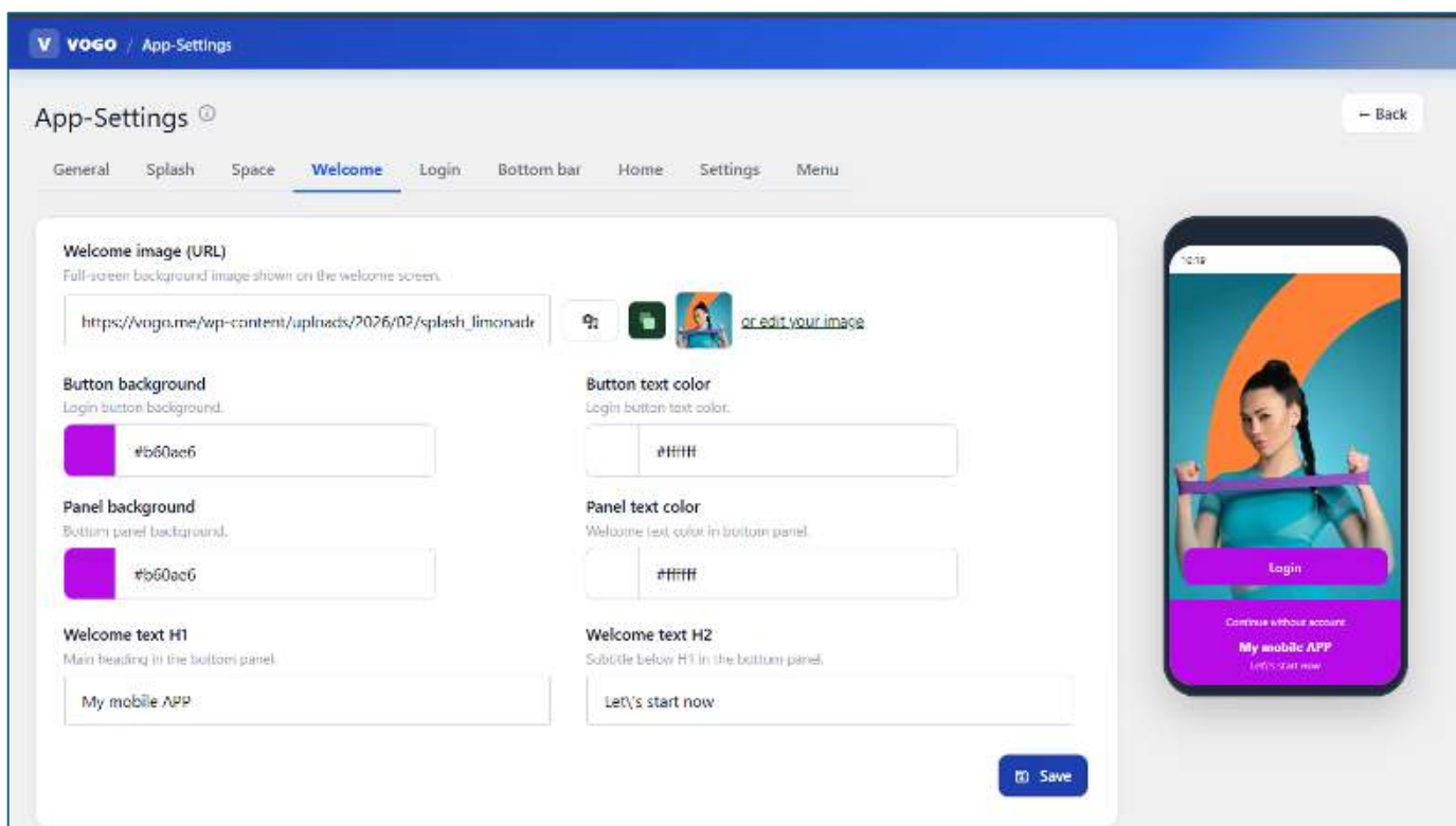
Fig. — Framework-ul VOGO® MAF — Mobile Application - App settings - Welcome screen cofiguration
